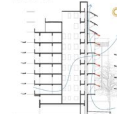
Section 01 Scale 1:300
