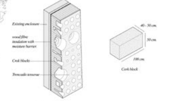
constructive detail Escal= 10
